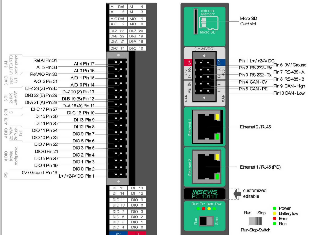
Figure Above: CPU and Periphery connectors of Panel-PLC PC1011T
