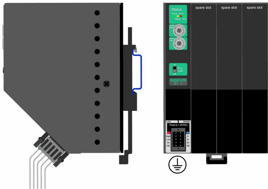
figure above: Sample of decentral head station DP303C from front side and from the side
